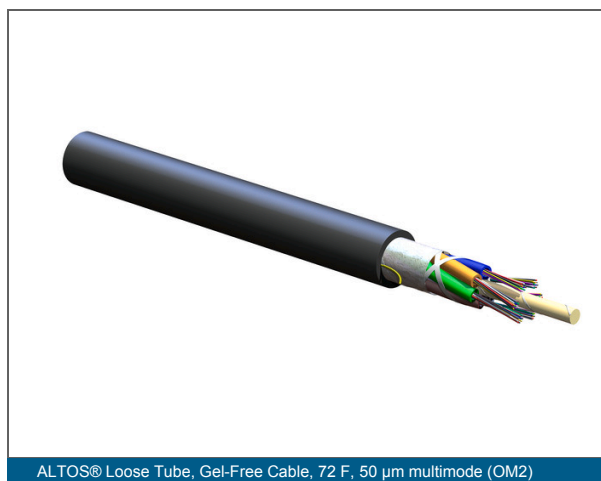
ALTOS® Loose Tube, Gel-Free Cable, 72 F, 50 µm multimode (OM2)
