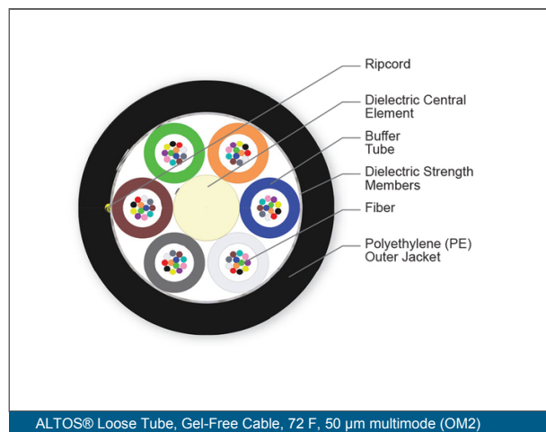
ALTOS® Loose Tube, Gel-Free Cable, 72 F, 50 µm multimode (OM2)
